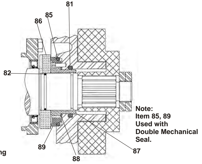
Mechanical Seal
