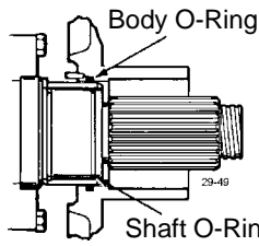
Figure 39 - Remove O-Rings
