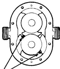
Apply gear puller here
